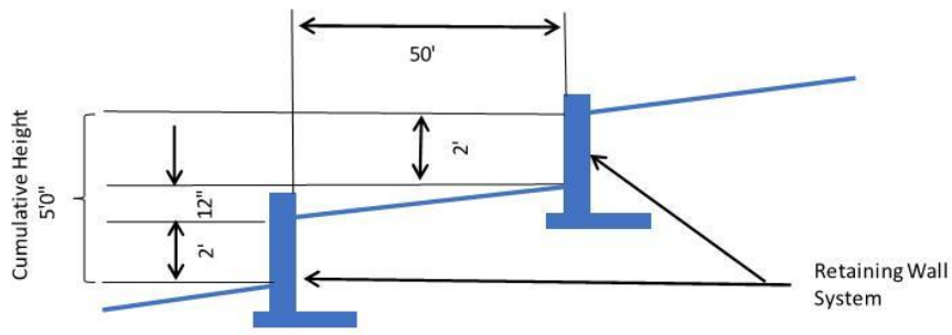
Example - B Design Professional Not Required
