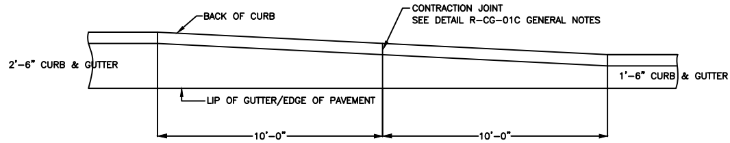
PLAN VIEW CURB TRANSITION 2'-6" CURB & GUTTER TO 1'-6" CURB & GUTTER
