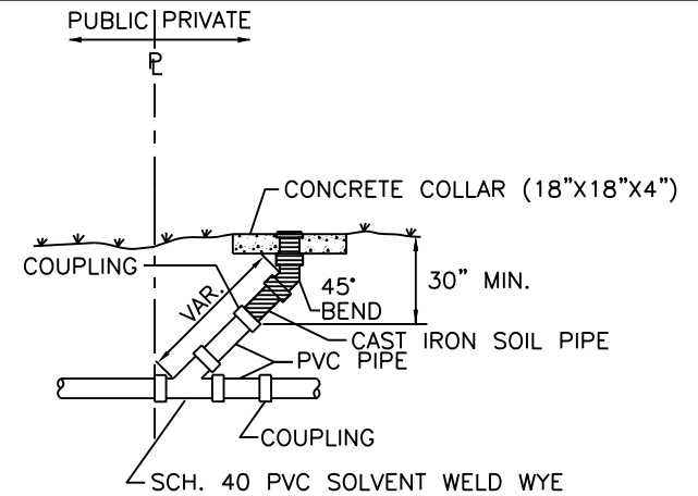
CLEAN OUT DETAILS INSTALLED BY PLUMBER
